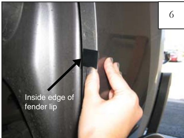
Center a supplied Tab (MT1-0002) over the marks made in step 4, aligning edge of tab with inside edge of fender lip (tab may extend over outside of fender).
