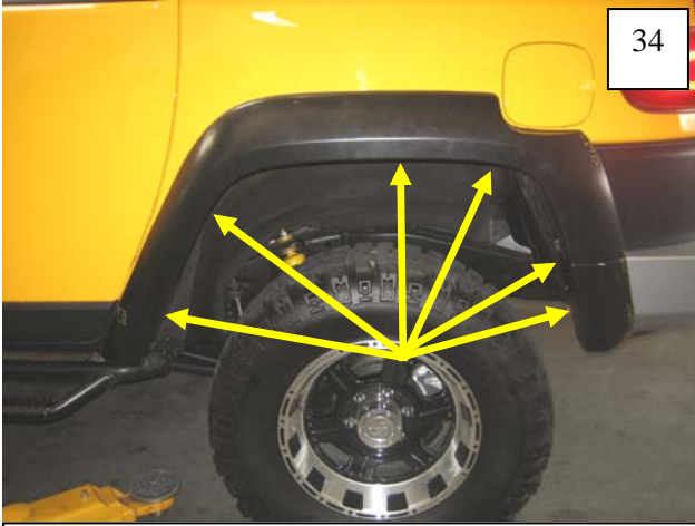
Position Flare on fender. Install six supplied #14 Hex Head Bolts. Do not tighten. NOTE: It is helpful to install one of the top screws first.
