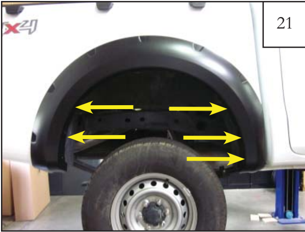
While holding Rear Flare onto vehicle using a #2 Phillips Screwdriver, start six (6) supplied Screws (SW1-0056) into flare and into clips installed in steps 17 & 18.
