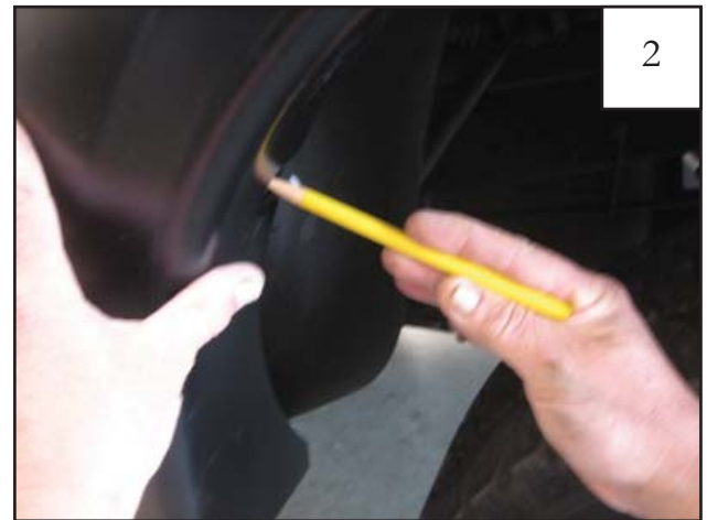
Hold flare to vehicle and mark four clip locations with a grease pencil. See Step 3 for locations.
