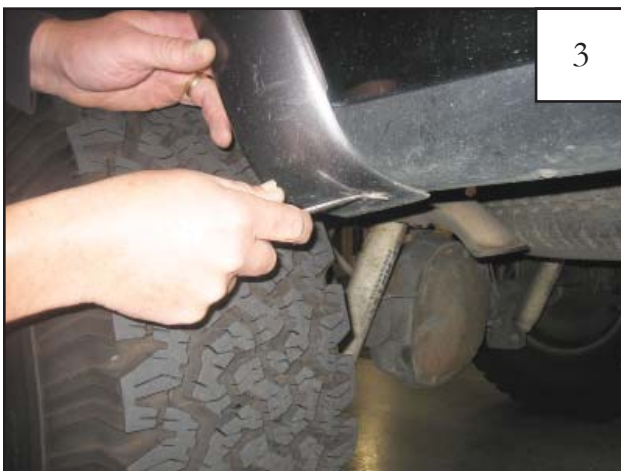
Use a trim tool to remove one plastic fastener located at bottom rear of wheel well as shown.
