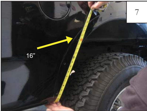
For trucks without factory flares ONLY: Wrapping tape measure up from underside of fender, measure up 16" and make a mark on fender lip where tape measure intersects.
