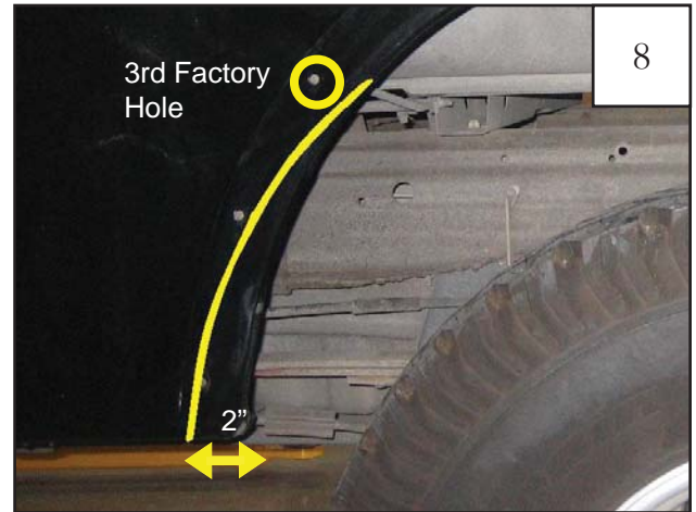
Draw a line from mark made in Step 5 up to mark made in Step 6 or Step 7, curving gradually to connect the marks. The line should be as shown.
