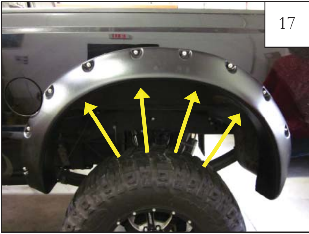
Using a #2 Phillips Driver, fasten screws (SW1-0015) through flare and inter inner fender using holes in flare as a guide.
