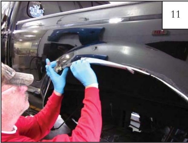
If needed, use tape to prevent caulk from dripping while drying.
