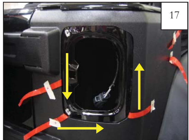
Tape liners 4, 5, & 6 may be removed in any order. Pull tape liner 4 downward. Pull tape liner 5 to the right. Pull tape liner 6 upward. NOTE: Refer to steps 8 & 9 for tape liner tab numbering.
