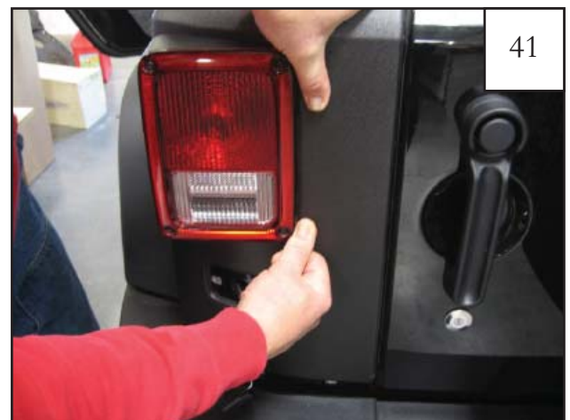
Once all tape liners are peeled, press down on entire again applying 30 PSI to the taped areas. Take special care in pressing down around the tail light. NOTE: The tape reaches maximum adhesive bond after 24 hours of contact. Do not wash vehicle for 24 hours.
