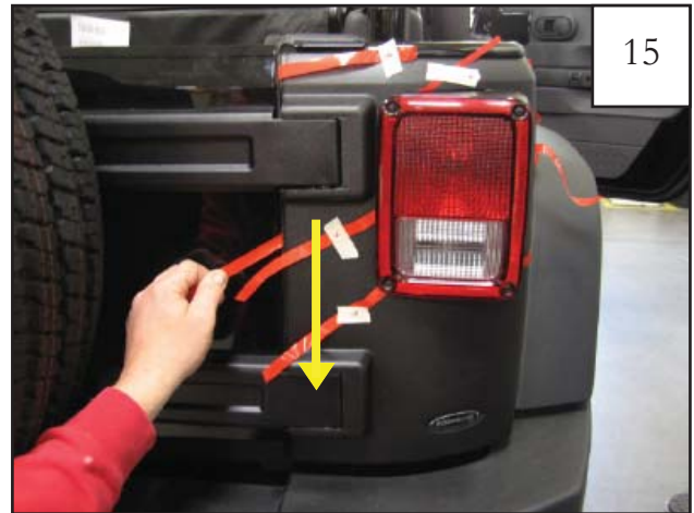
Pull tape liner 2 downward. NOTE: Refer to steps 8 & 9 for tape liner tab numbering. Using a #2 Phillips screwdriver, remove the light again.
