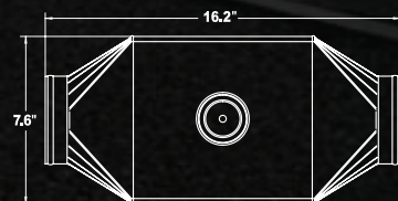
#9804 4" ULTRA LOW 180° ANGLE
