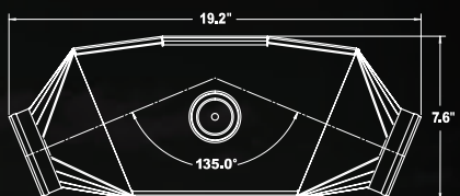
#9834 4" ULTRA LOW 135° ANGLE
