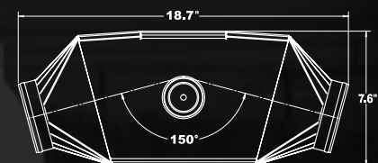
#9854 4" ULTRA LOW 150° ANGLE
