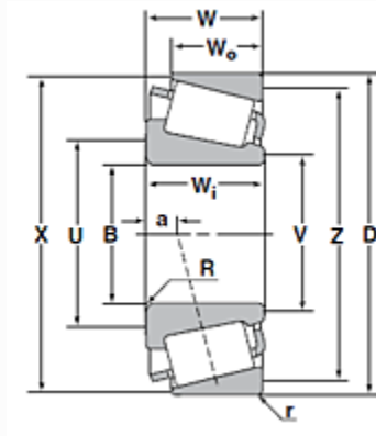
Cup for Tapered Roller Bearing - Inch Series and J Series - Dimensions
