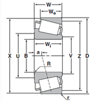
Cup for Tapered Roller Bearing - Inch Series and J Series - Dimensions
