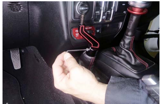
18. Apply medium strength thread locking fluid to cap screw (4) and install it in the shift handle.
