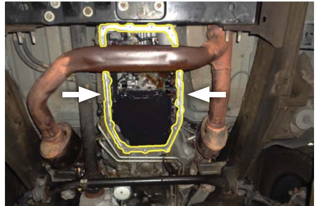
15. Use lint free rag to clean transmission pan mounting surface.
