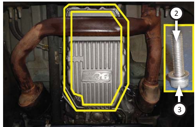
16. Install deep pan with 25MM screws (x15) (2) and flat washers (x15) (3) hand-tight. Then torque screws to 8ft lbs.
