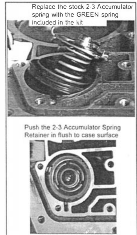
Figure 7. 2-3 Accumulator Assembly
