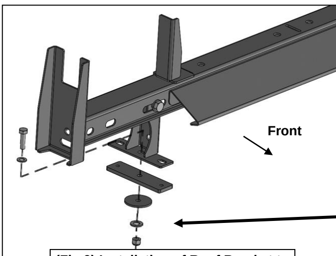
(Fig 9) Installation of Roof Bracket to roof for Transit Connect illustrated
