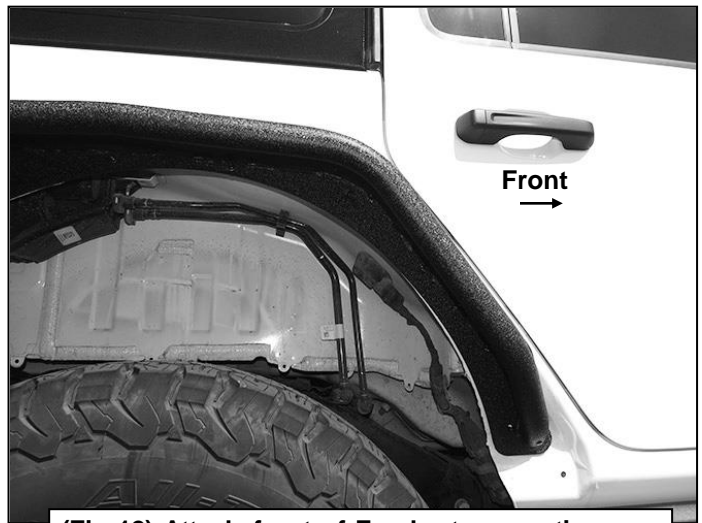
(Fig 12) Attach front of Fender to mounting locations on body, (passenger/right Fender)
