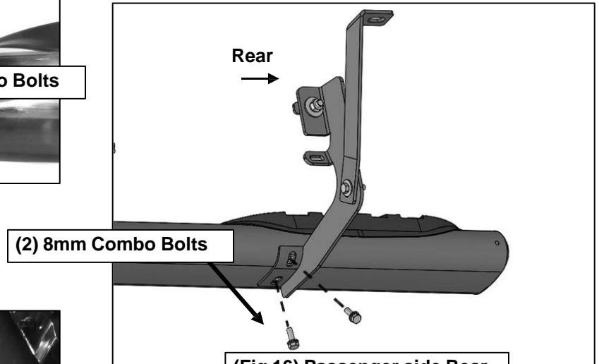
(Fig 16) Passenger side Rear Bracket attached to Sidebar
