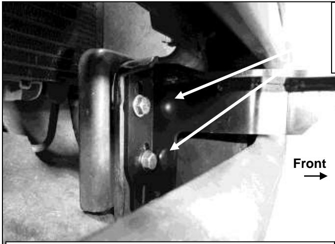
(Fig 5) 2006-08 driver side Top Bracket installation
