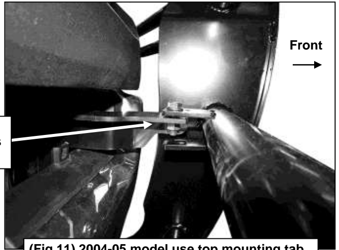
(Fig 11) 2004-05 model use top mounting tab
