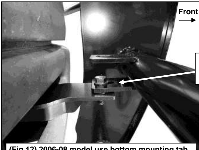
(Fig 12) 2006-08 model use bottom mounting tab
