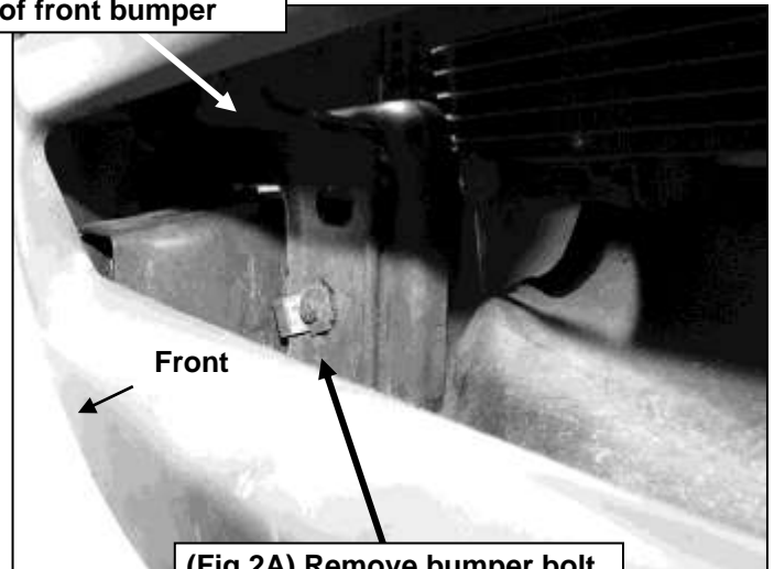
(Fig 2A) Remove bumper bolt (2006-08 model pictured)
