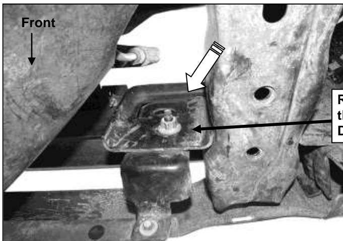
(Fig 2B) Remove hex nuts from bumper bolt (06-08 passenger side pictured from below/behind bumper)
