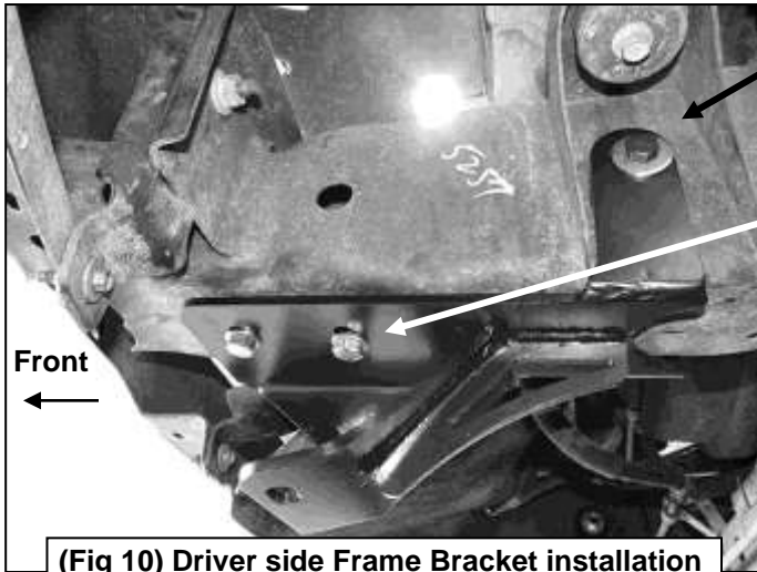
(Fig 10) Driver side Frame Bracket installation (model w-o tow hook)
