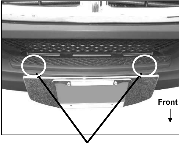
(Fig 4) Remove (2) factory screws (Torx head)
