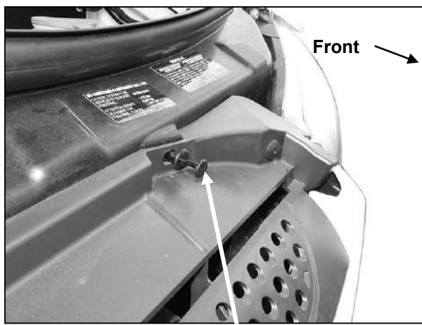
(Fig 16) 2015-16 models, remove top outer plastic clip (driver/left side pictured)
