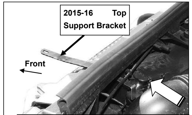
(Fig 17) Insert 8mm "Z" Bolt Plate through back of radiator cross member (arrow)
