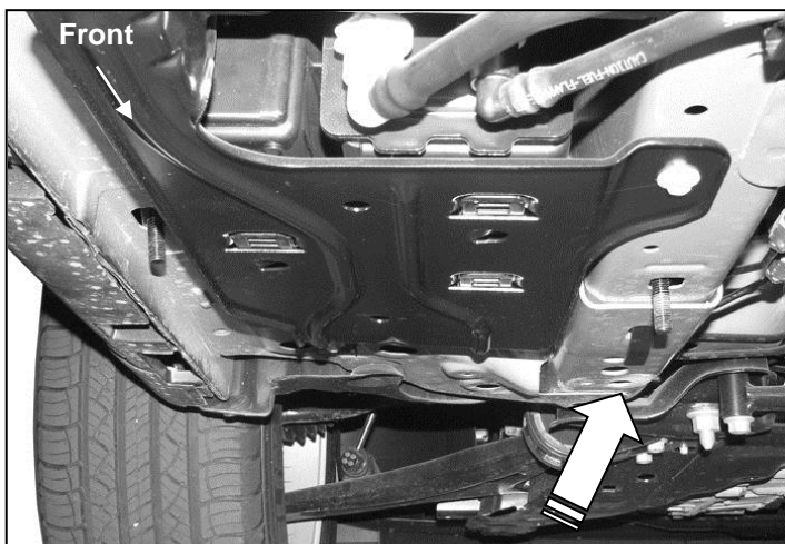
(Fig 3B) Insert Bolt Plate into the oval hole and out the square hole in bottom of inner frame channel
