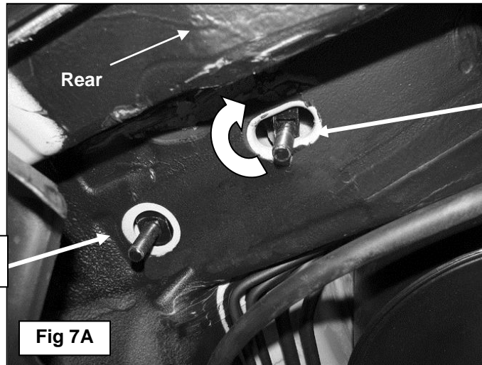
10mm x 40mm T-Bolt Plate Insert T-Bolt Plate into opening and rotate 90-degrees to direction of slot
