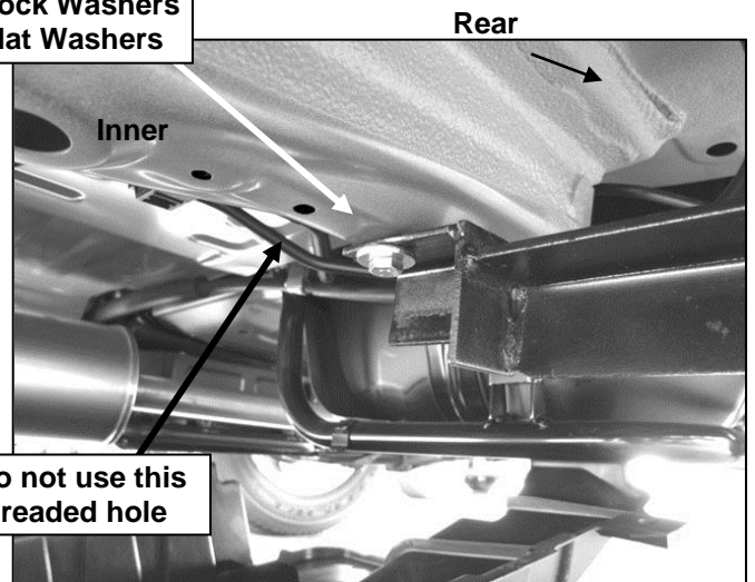
(Fig 7) Driver Side Rear Mounting Bracket Pictured
