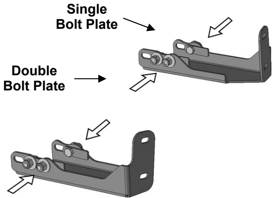
(Fig 12) Typical Silverado/Sierra mounting position with Brackets "IN" toward vehicle
