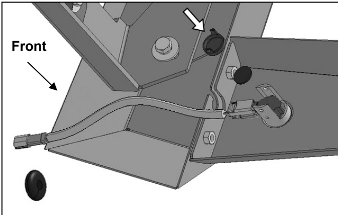
(Fig 19) Slide sensor into sleeve, insert Foam Washer and Clip to lock sensor in sleeve
