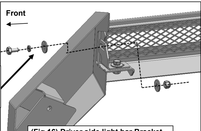
(Fig 16) Driver side light bar Bracket attached to Mesh hardware
