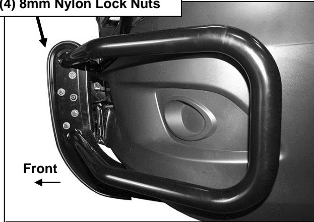
(Fig 11) Bolt Wing to Center Section (optional)
