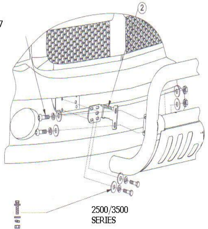
FIGURE 3-INSTALLATION VIEW OF PASSENGER SIDE, DRIVER SIDE OPPOSITE
