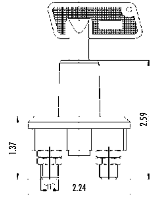
Measurements are in inches
