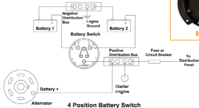
4 Position Battery Switch
