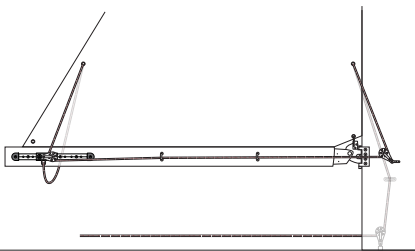
Single line reefing
