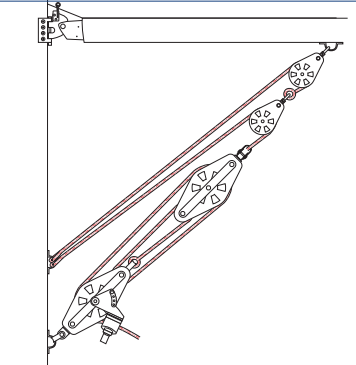
16:1 Cascaded kicker
