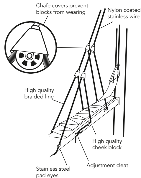
Blocks, cleats, mounting eyes and fixings included in the kit.
