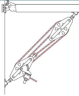
4:1 Split backstay
