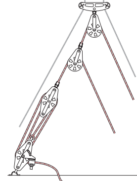
16:1 Split backstay
