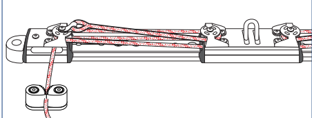
4:1 Remote cleats
