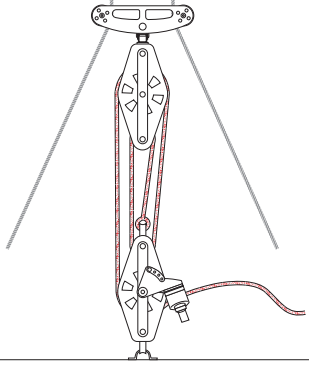
4:1 Split backstay
