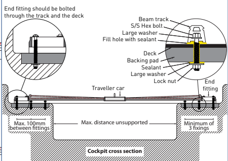
Beam track fitting
