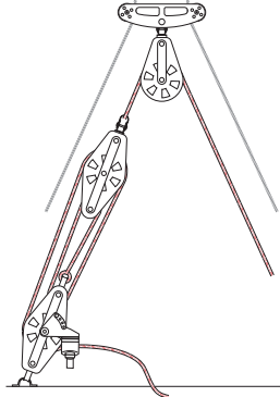
8:1 Split backstay
