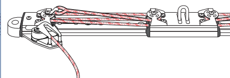
4:1 Traveller cleats on end
