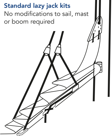
Blocks, cleats, mounting eyes and fixings included in the kit.
