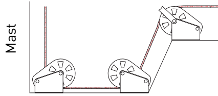
Over the top
