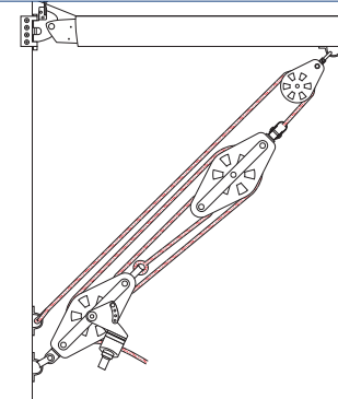
8:1 Cascaded kicker
