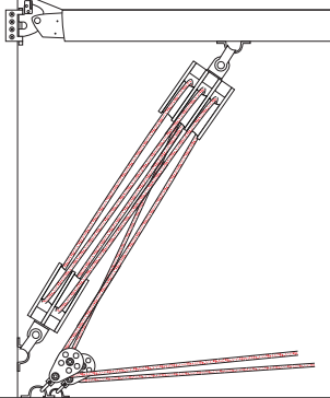
Kicker 6:1 led aft
