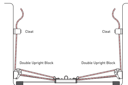
3:1 Remote cleat
