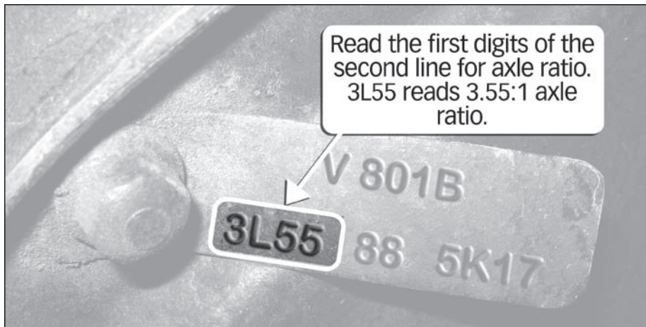
Figure 5 Axle Ratio Tag Bolted on Rear Differential
