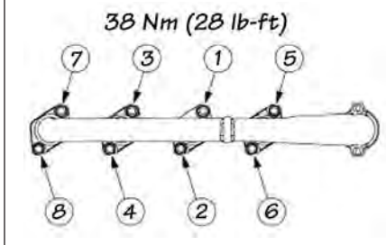
Figure 25: Exhaust manifold tightening sequence
