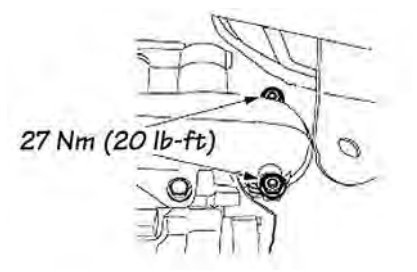
Figure 26: Turbocharger adapter pipe torque specification
