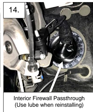
Firewall Passthrough
