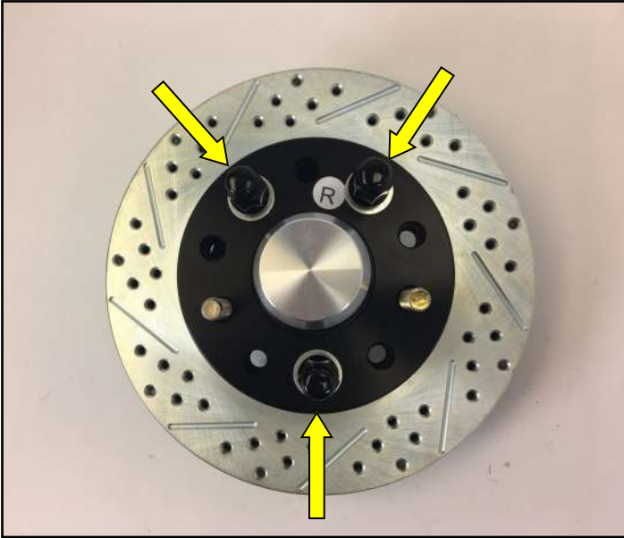
5. Install the correct side rotor onto the hub and secure with 3 lug nuts and washers to avoid scratching the hat.
