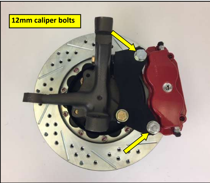
7. Inboard view of caliper installed. Once correct shimming is achieved, torque the 12mm caliper bolts to 85ft lbs.
