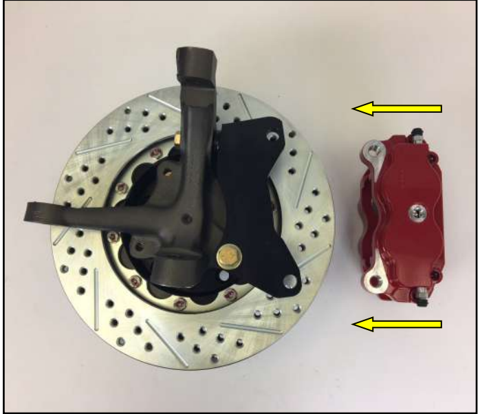
6. Install the caliper onto the rotor using the supplied 12mm bolts and washers. Tighten these snug as you may need to remove for the shimming process. Check to make sure the caliper does not come in contact with the rotor once secured.
