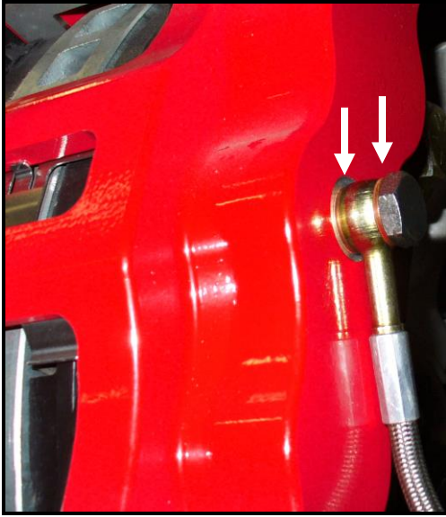
Figure 4: Brake hose installed into caliper with banjo bolt and washers
