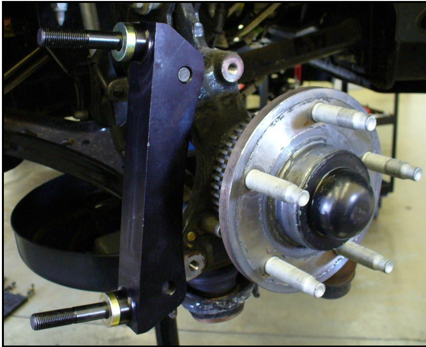
Figure 3: Radial bracket installed onto the passenger side spindle with spacers
