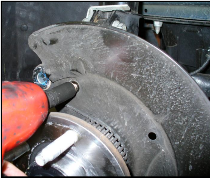
Figure 1: Removal of dust shield (passenger side)
