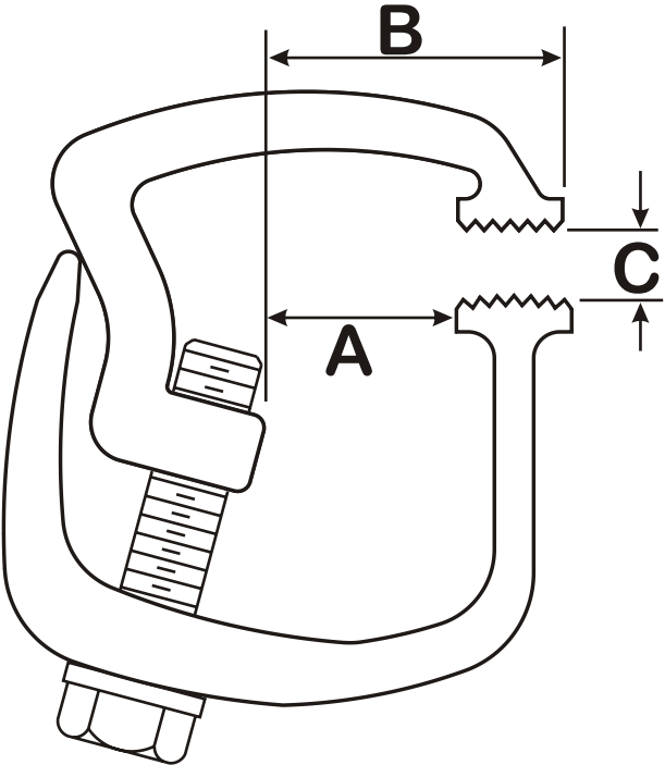
Clamp Width 1-1/4"
