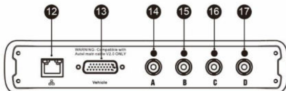
Figure 2-7 VCMI Bottom View
