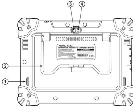
Figure 2-2 MaxiSys Tablet Back View
