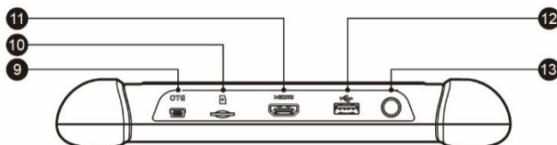
Figure 2-3 Display Tablet Top View
