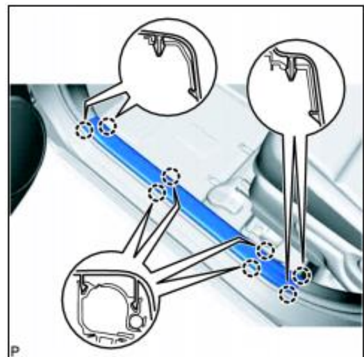
Picture 9: Front LH scuff plate
