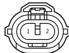
Picture 6: Factory Fog Light harness. Pin 1: Negative Pin 2: Positive
