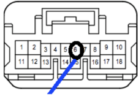
Picture 25A DRL's blue wire to connector If1, pin 6, red wire (5A panel fuse)
