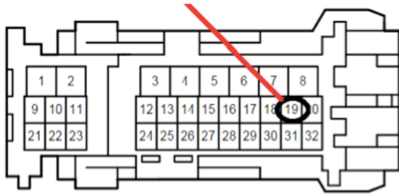
Picture 24B: DRL's red wire to connector 4F, Pin 19, black wire (10A Ignition Fuse No3)
