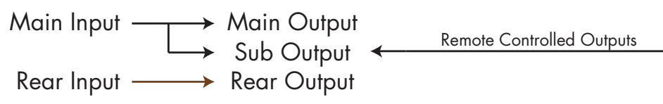
Two Linked Channels / One Independent Channel All Connected to Main LEDs OFF
