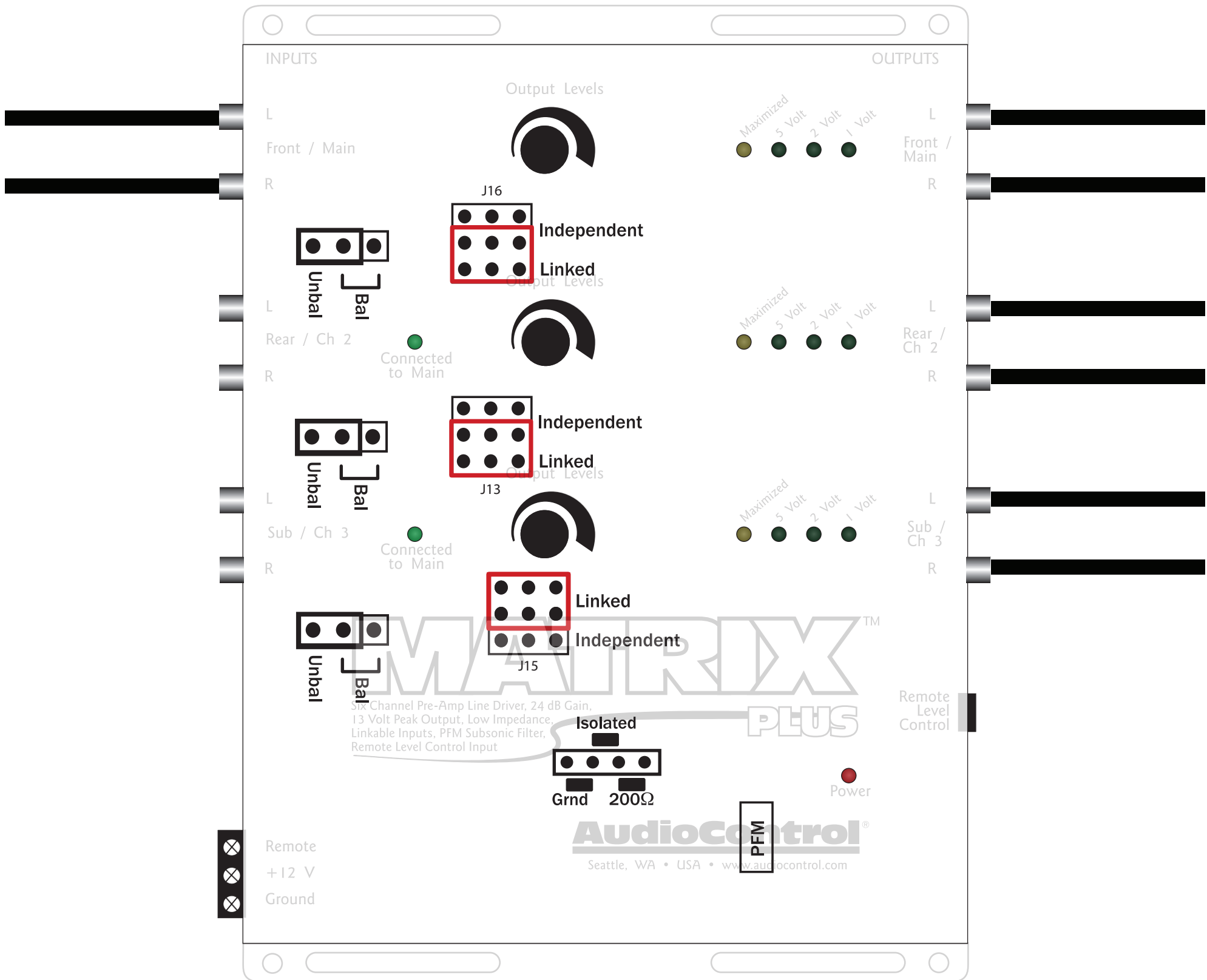
Three Linked Channels All Connected to Main LEDs ON
