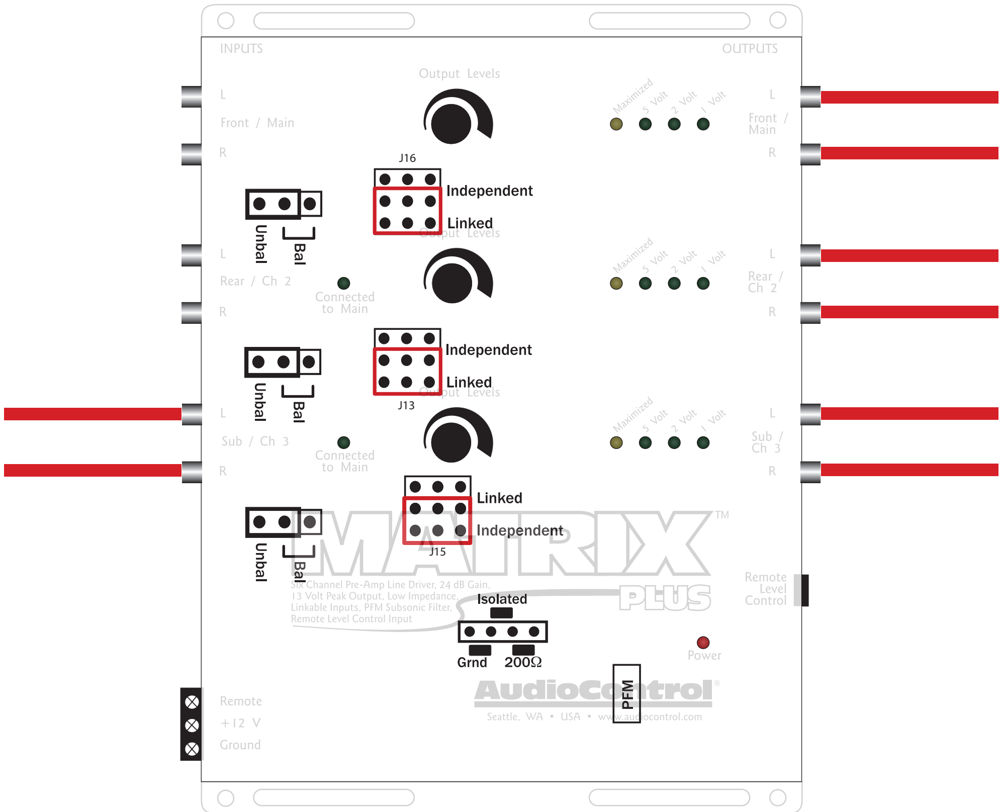
Three Linked Channels All Connected to Main LEDs OFF
