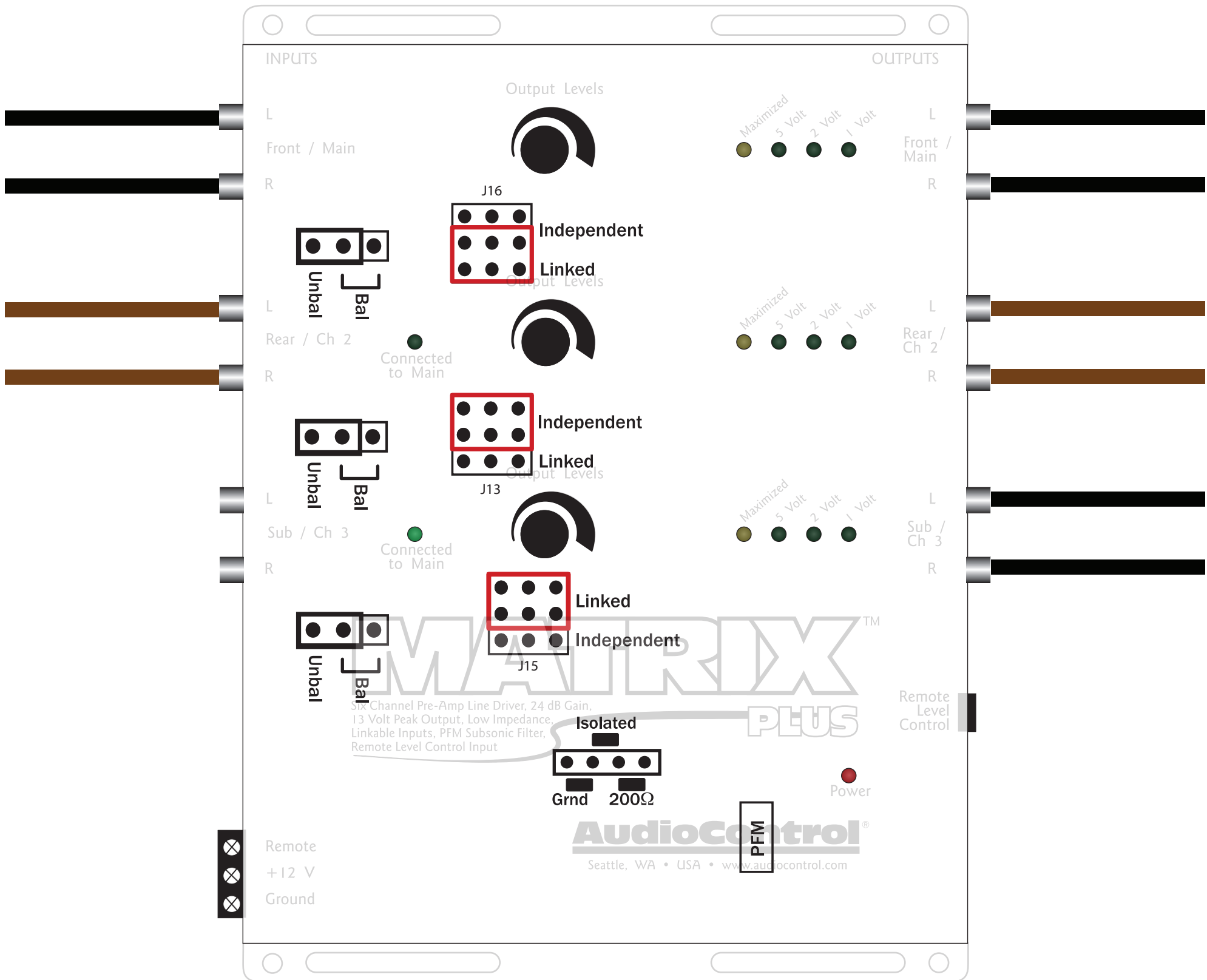
Two Linked Channels / One Independent Channel Sub Connected to Main LED On
