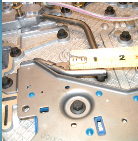
1-1/4" from bend
