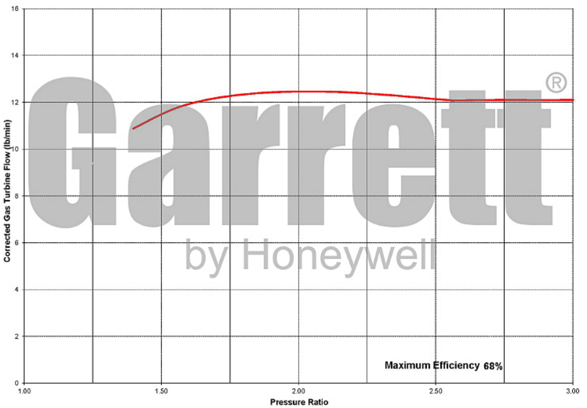
GT1749V, 70 Trim, 0.61 A/R
