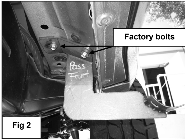
Front Passenger Side Mounting Bracket
