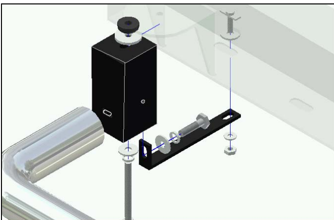
Figure 1.4 – 1500 Front Mount Assembly
