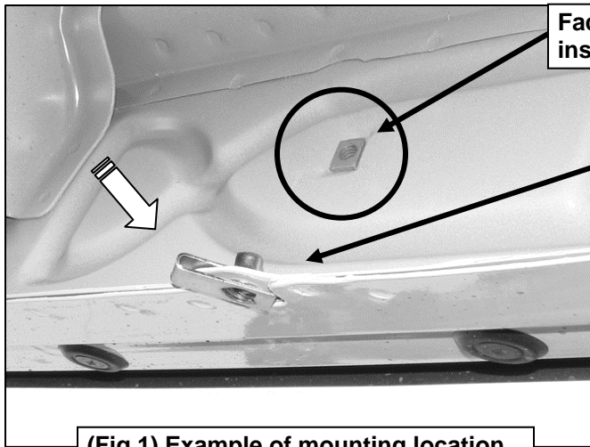
(Fig 1) Example of mounting location, (top), with factory threaded hole
