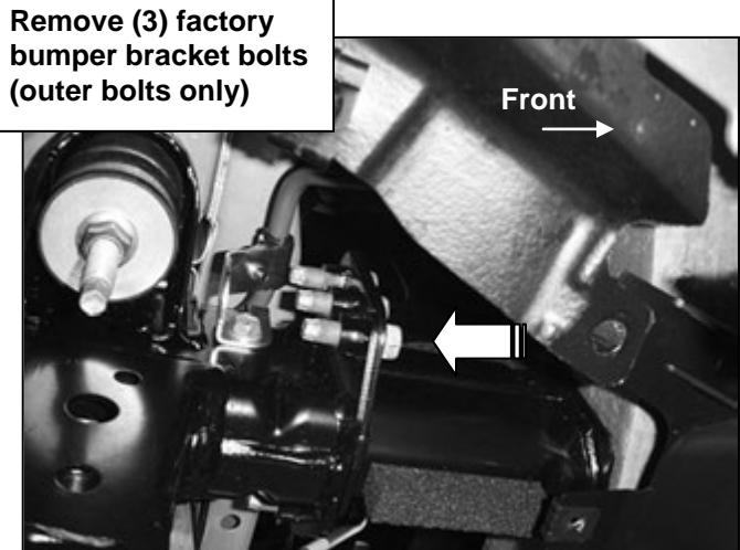
(Fig 3) Passenger side pictured from below vehicle
