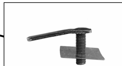
(Fig 3A) 10mm Bolt Plate
