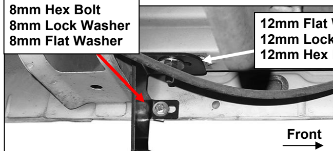
(Fig 9) Driver/left side rear Bracket installation
