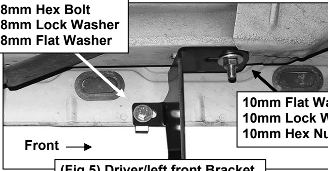
(Fig 5) Driver/left front Bracket
