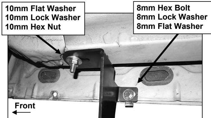
(Fig 15) Passenger/right front Bracket
