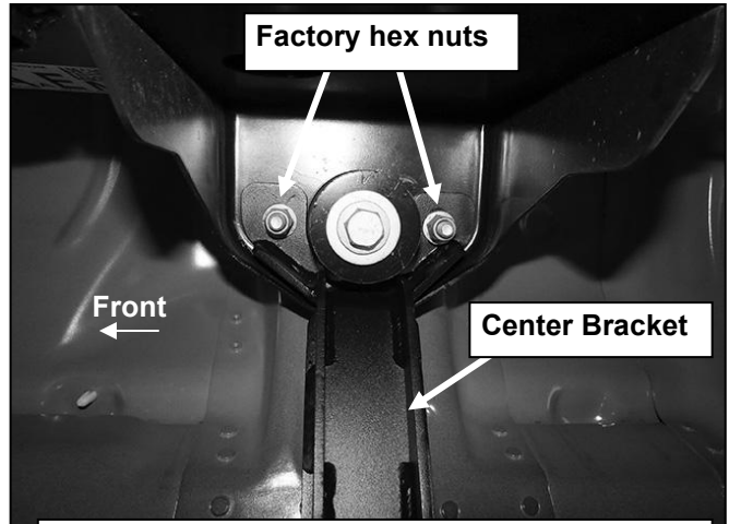
(Fig 6) Reuse factory hex nuts to attach center Bracket to underside of center body mount
