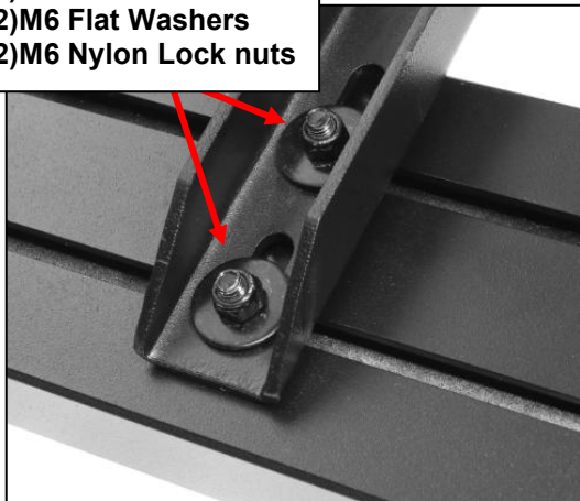
(Fig 9) Passenger side Bracket installed
