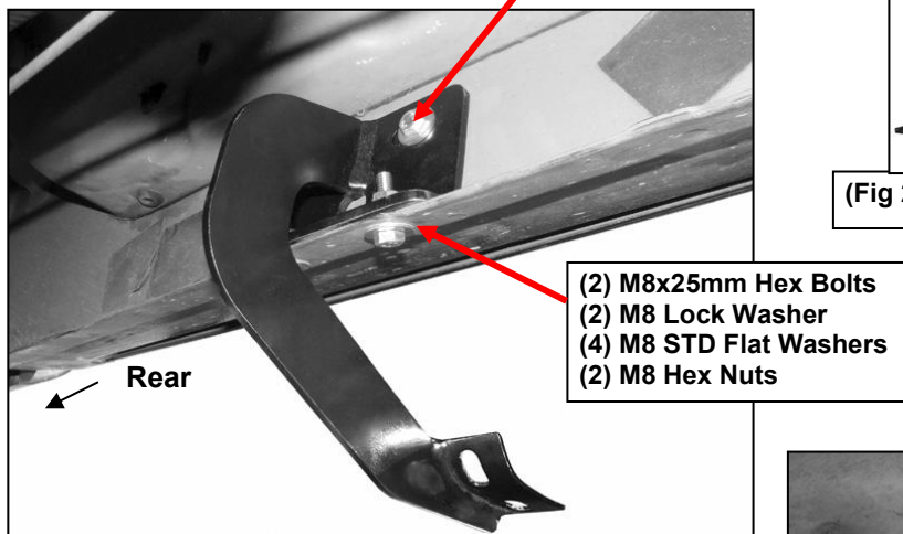
(Fig 3) Driver side-rear Mounting Bracket location
