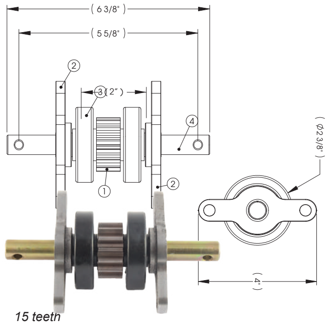
014-281331 - 2x2 Gear Pack (Without roll pin assy.)
