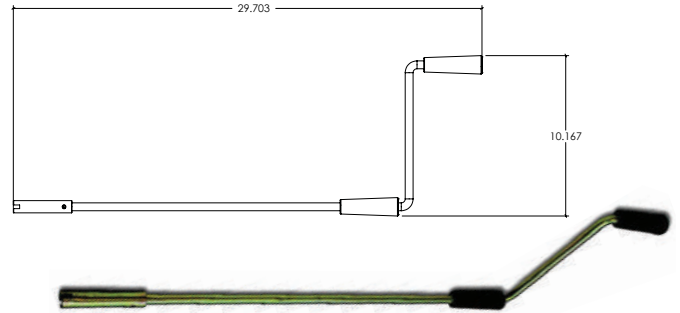
014-119226 - Standard S/O Crank Handles
