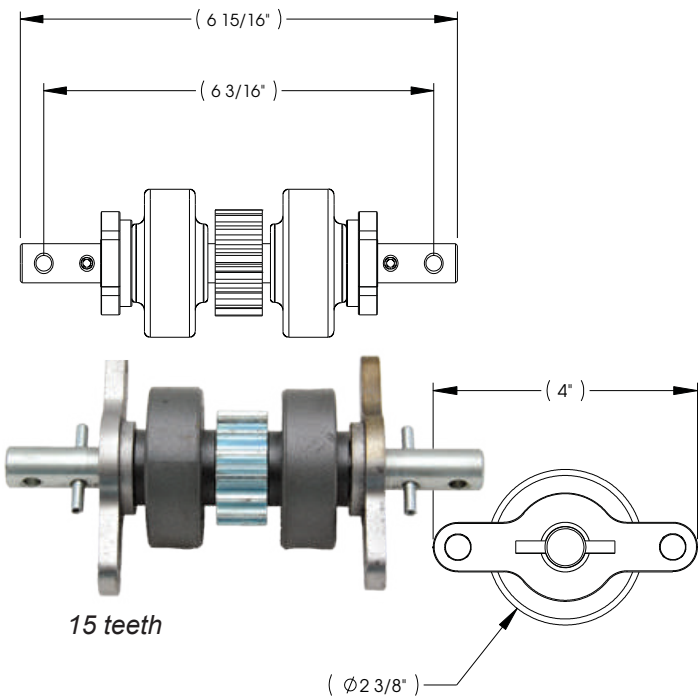
014-140409 - Gear Pack 2x3 (With roll pin assy.)
