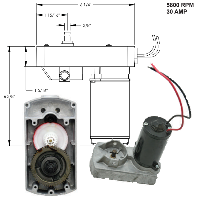
014-136373 - 28:1 Venture Actuator Motor (2-1/2" inner gear)
