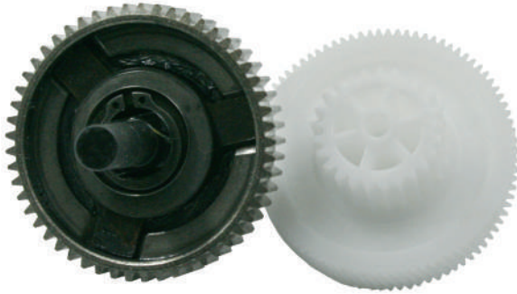
014-191072 - 18:1 Venture Gear Set
