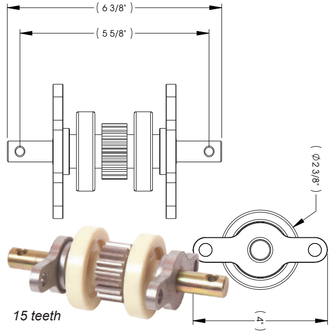
014-324869 - Standard Gear Pack - nickel (Without roll pin assy.)
