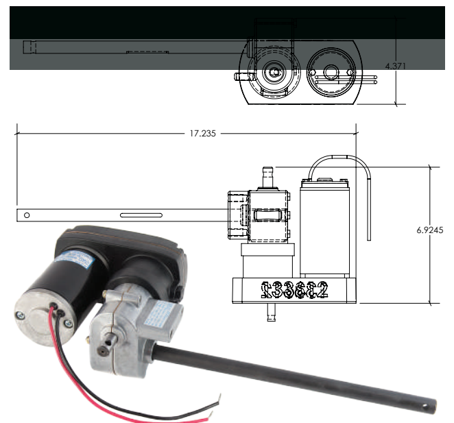
014-133612 - 18:1 Tuscon Motor/Driveshaft (With right angle gear box)
