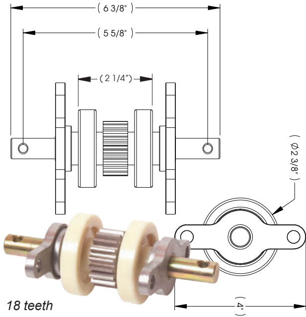
014-122837 - Standard Gear Pack - nickel (Without roll pin assy.)
