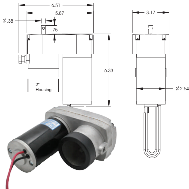
014-125802 - 9000 RPM 18:1 Motor (Tuscon) (When not avail. sub. with 014-168956)
