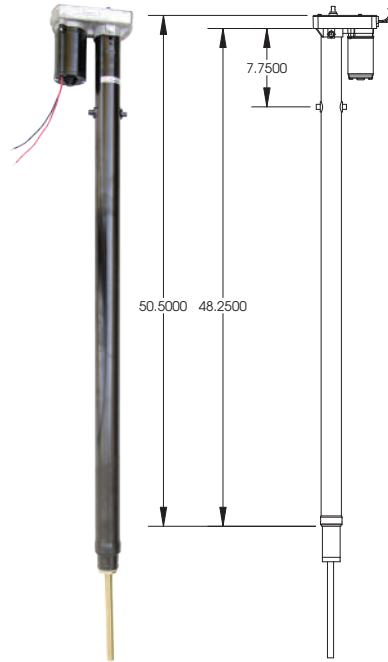
014-168956 - 40" Venture Actuator - High Speed Motor
