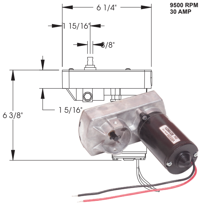
014-132682 - 18:1 Venture Actuator Motor (2-1/4" inner gear)
