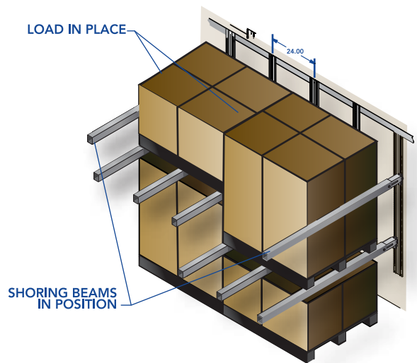
SINGLE & DOUBLE SYSTEM ON 24-IN. CENTERS (DOUBLE-SINGLE-DOUBLE) + Ability to deck at multiple heights
