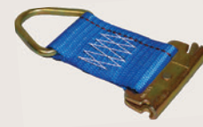
40386-11 Series E and A Rope Tie Off Spring actuated fitting for use with Series E or Series A Track. WLL: 1,333 lbs./605 kg. Weight: .40 lbs./0.18 kg.
