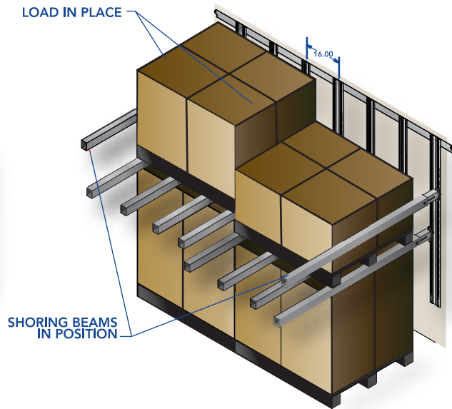
SINGLE & DOUBLE SYSTEM ON 16-IN. CENTERS (DOUBLE-SINGLE-SINGLE-DOUBLE) + Ability to deck at multiple heights
