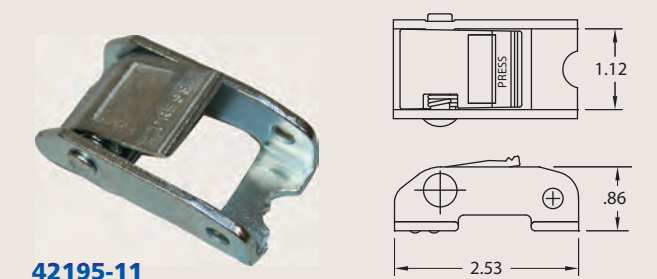
42195-11 WLL: 500 lbs./227 kg. Weight: .25 lb./11 kg.
