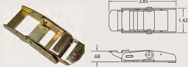
42816-18 WLL: 600 lbs./272 kg. Weight: .15 lb./06 kg.
