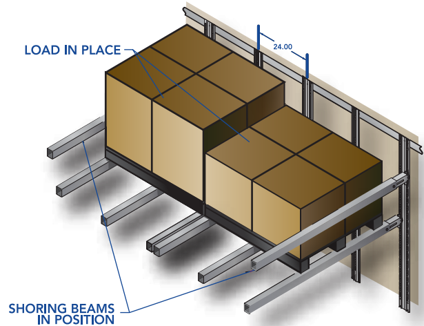
SINGLE & DOUBLE SYSTEM ON 24-IN. CENTERS (DOUBLE-SINGLE-DOUBLE) + Pallets rest on 3 individual beams
