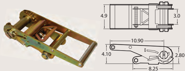
48965-10 WLL: 7,333 lbs./3,333 kg. Weight: 7.0 lbs./3.18 kg.
