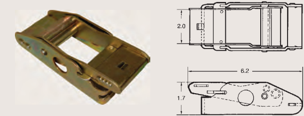
44639-12 WLL: 1,666 lbs./757 kg. Weight: 1.20 lbs./54 kg.
