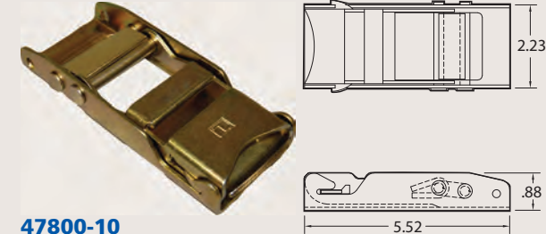
47800-10 WLL: 1,666 lbs./757 kg. Weight: .70 lb./31 kg.
