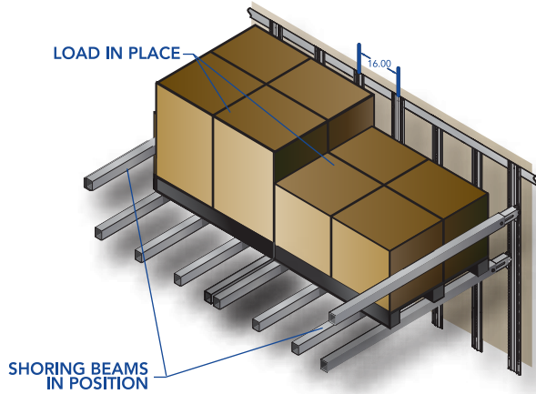
SINGLE & DOUBLE SYSTEM ON 16-IN. CENTERS (DOUBLE-SINGLE-SINGLE-DOUBLE) + Pallets rest on 4 individual beams
