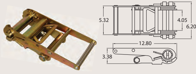
49349-10 WLL: 8,000 lbs./3,636 kg. Weight: 8.0 lbs./3.63 kg.
